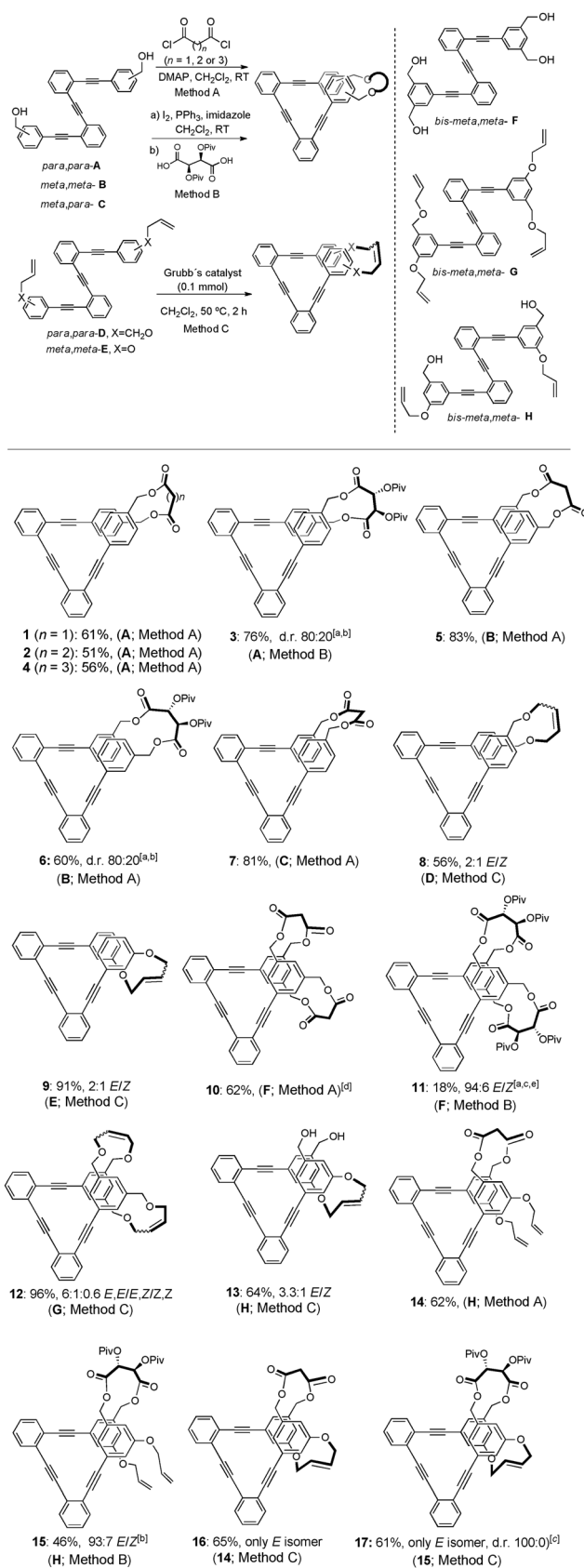
Scheme 1. Synthesized CNCs 1–17 from o -PEOs A–H . [a] Yield based on recovered starting material. [16] [b] Chiralpack IC column using n -hexane/ i PrOH (90:10) as the eluent with a 0.5 mL min −1 flow rate. [c] Chiralpack IB column using n -hexane/ i PrOH (90:10) as the eluent with a 0.5 mL min −1 flow rate. [d] Used 2 equiv of malonyl chloride. [e] Used 2 equiv of (–)- O,O' -di-pivaloyl-L-tartaric acid.
