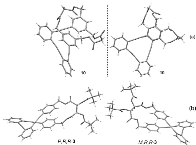
Figure 1. Representative X-ray structures: a) 10 (side view left and top view right). b) P,R,R - 3 and M,R,R - 3 . [27]
