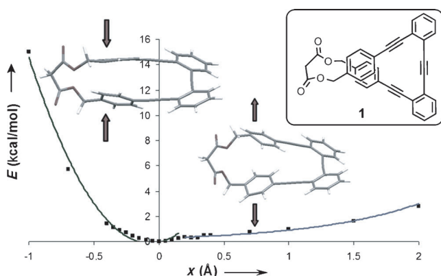
Figure 3. Potential energy profile of compound 1 toward elongation.
