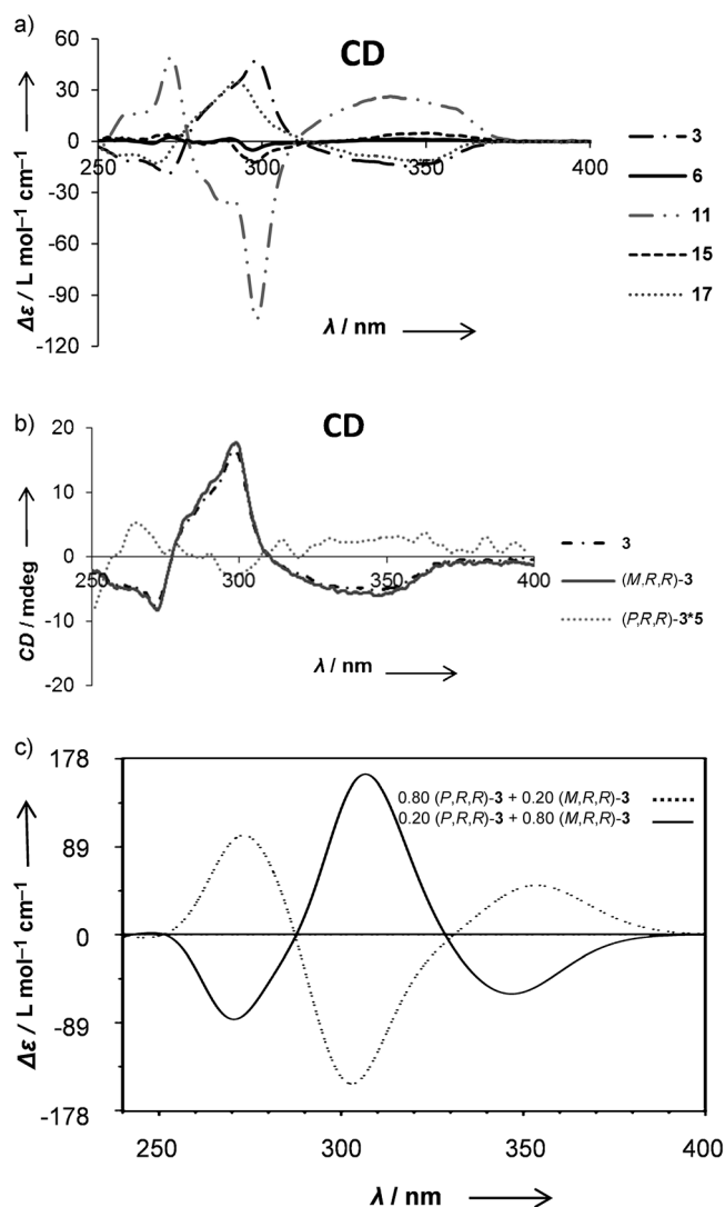
Figure 2. CD spectra ( 1 \times 10^{-5} M in \text{CH}_2\text{Cl}_2 ). a) Mono and doubly stapled derivatives (–)- 3 , (+)- 6 , (+)- 11 , (+)- 15 , and (–)- 17 . b) Pure diastereomers ( M,R,R )- 3 (solid line) and ( P,R,R )- 3 (dotted line), 80:20 mixture of ( M,R,R )- 3 and ( P,R,R )- 3 (dash-dot line). c) TD-PBE0/6-31G* spectra [25] of ( M,R,R )- 3 / (P,R,R) - 3 (80:20; solid line) and ( P,R,R )- 3 / (M,R,R) - 3 (80:20; dotted line).
